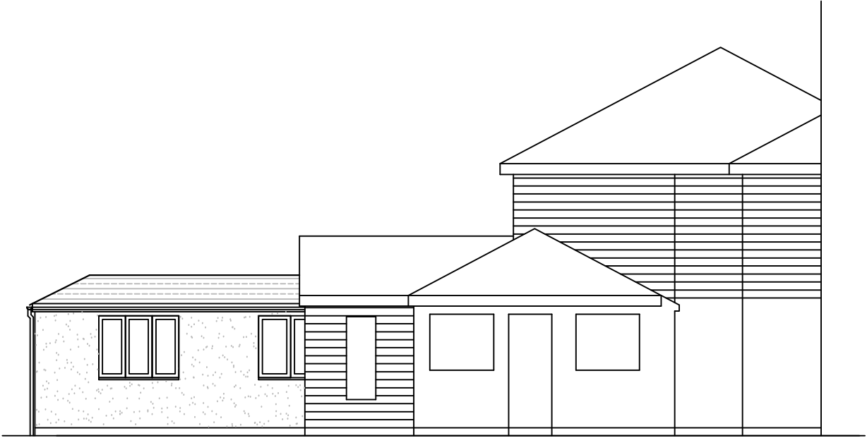
Part Proposed Side Elevation (West)
