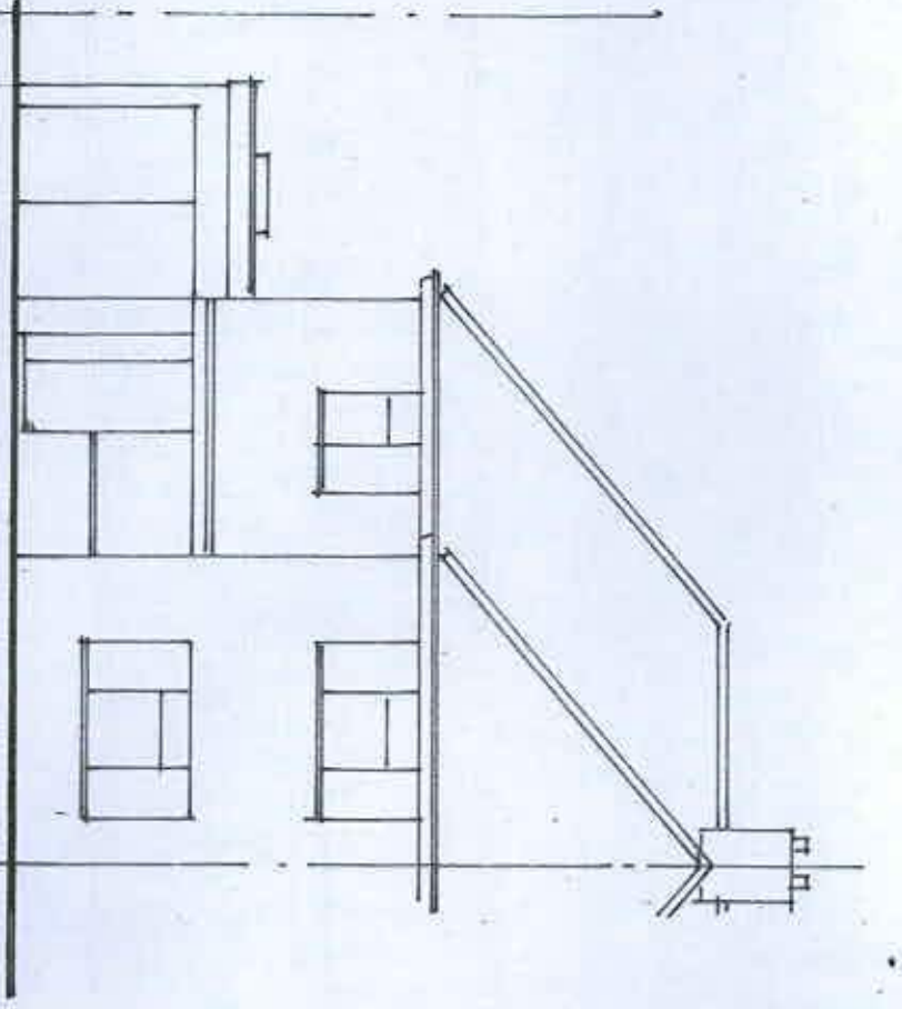
FRONT ELEVATION 1-100
