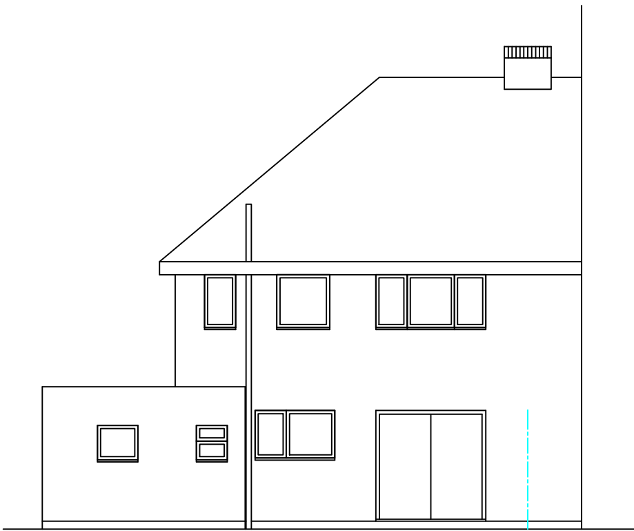
Existing Rear Elevation (South)
