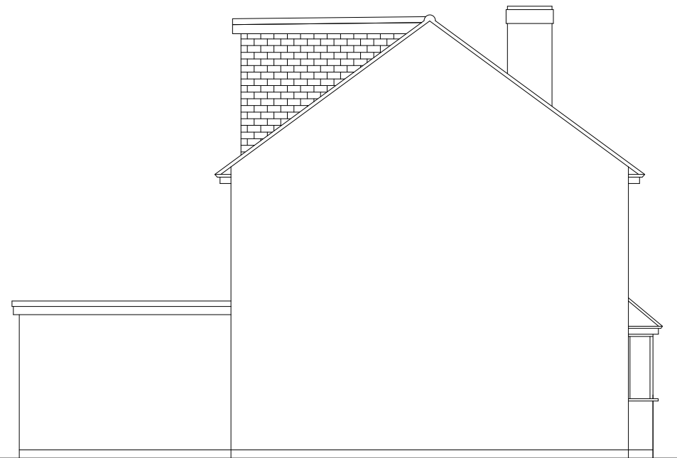
NEW SOUTH ELEVATION
