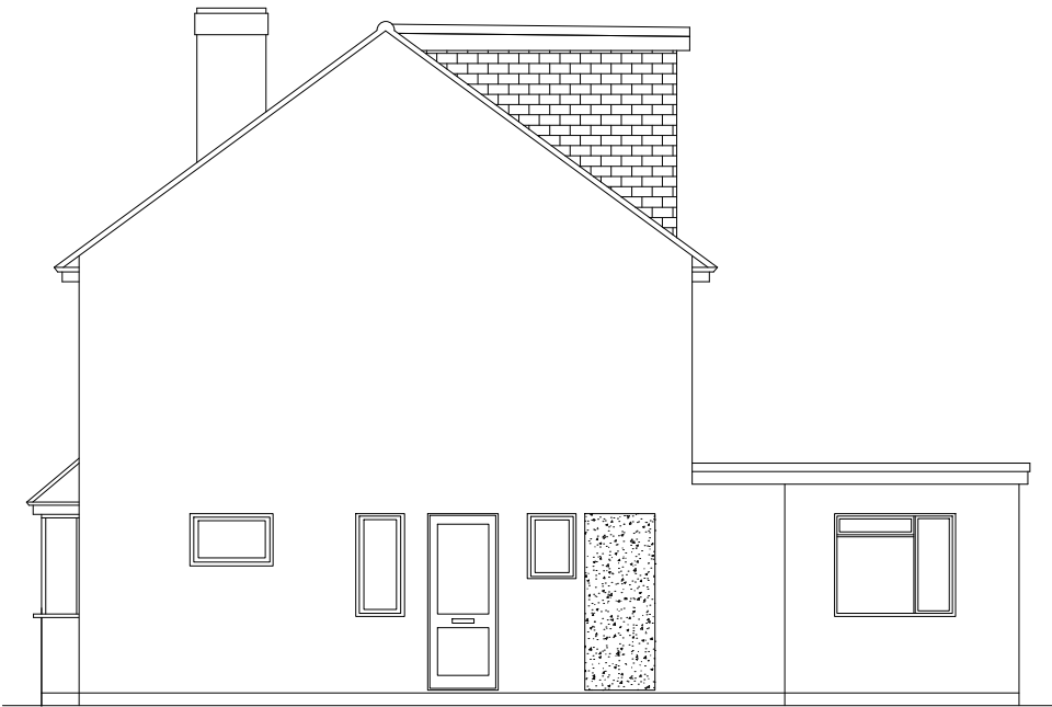
NEW NORTH ELEVATION
