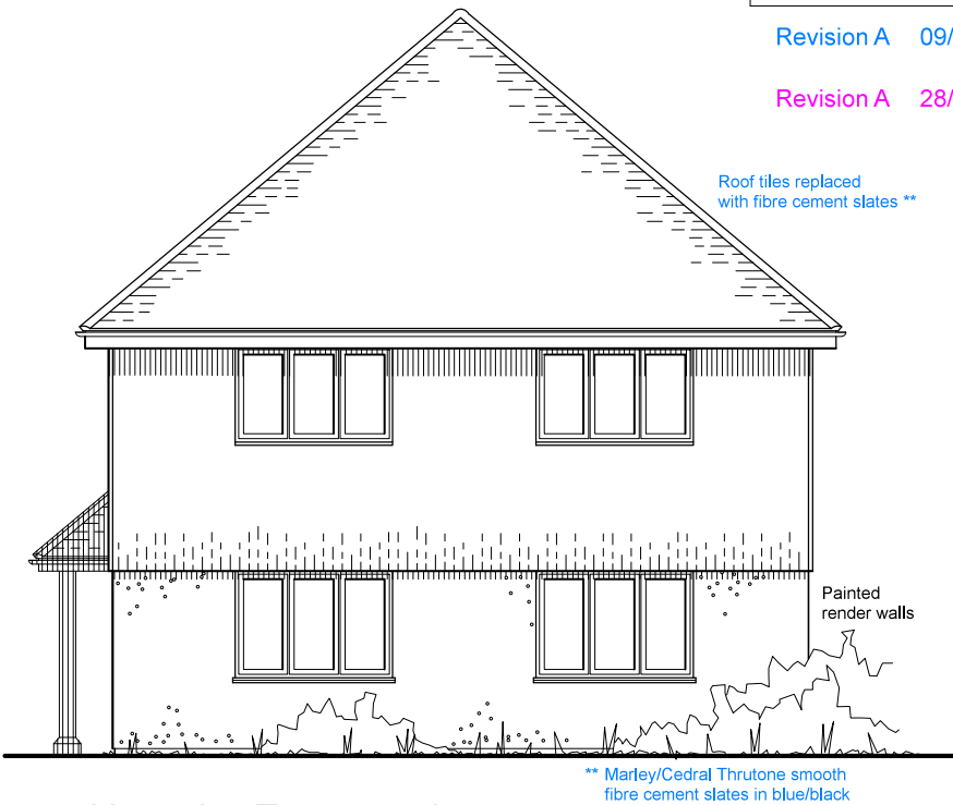
North Elevation
