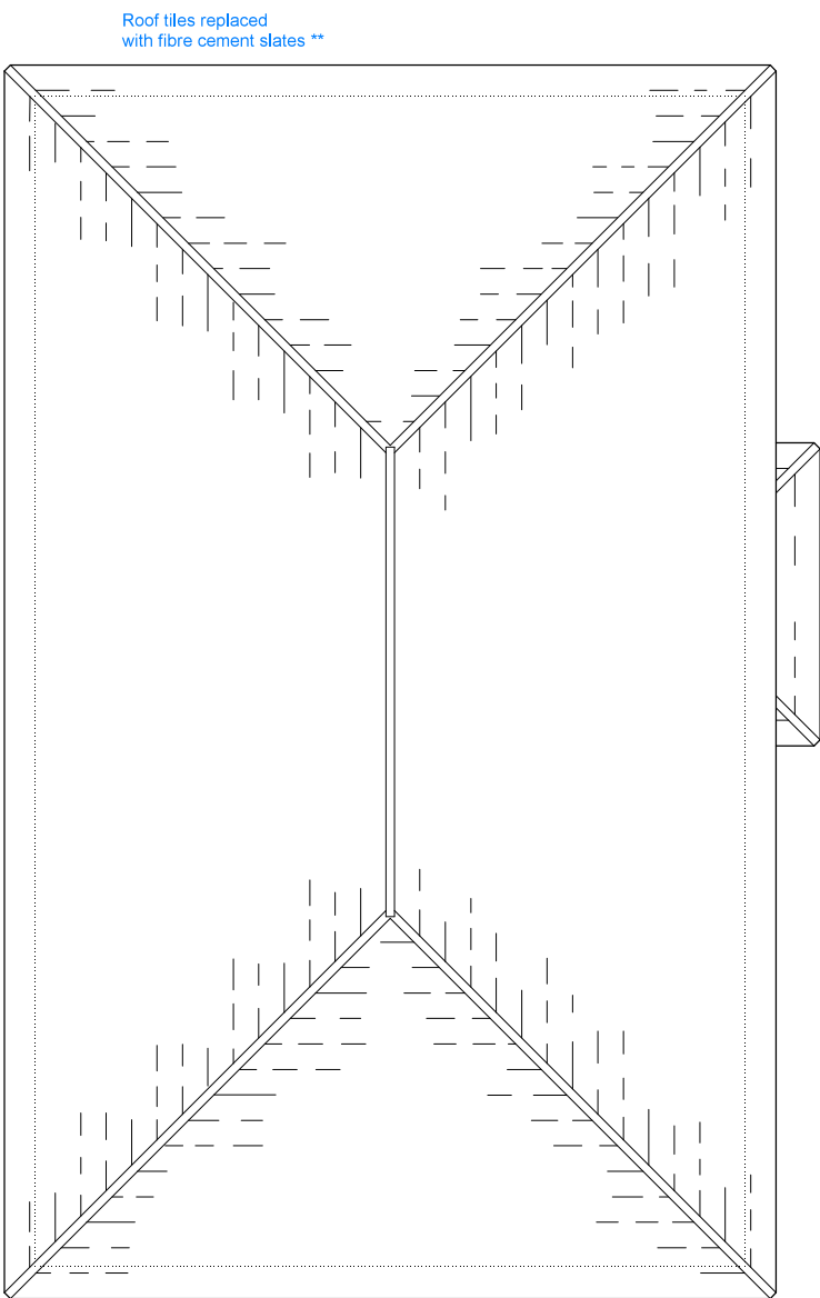
Roof Plan
