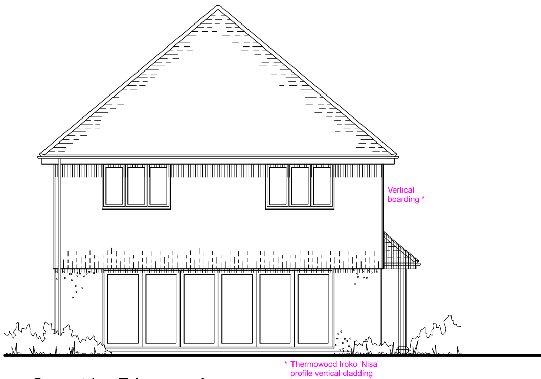
South Elevation
