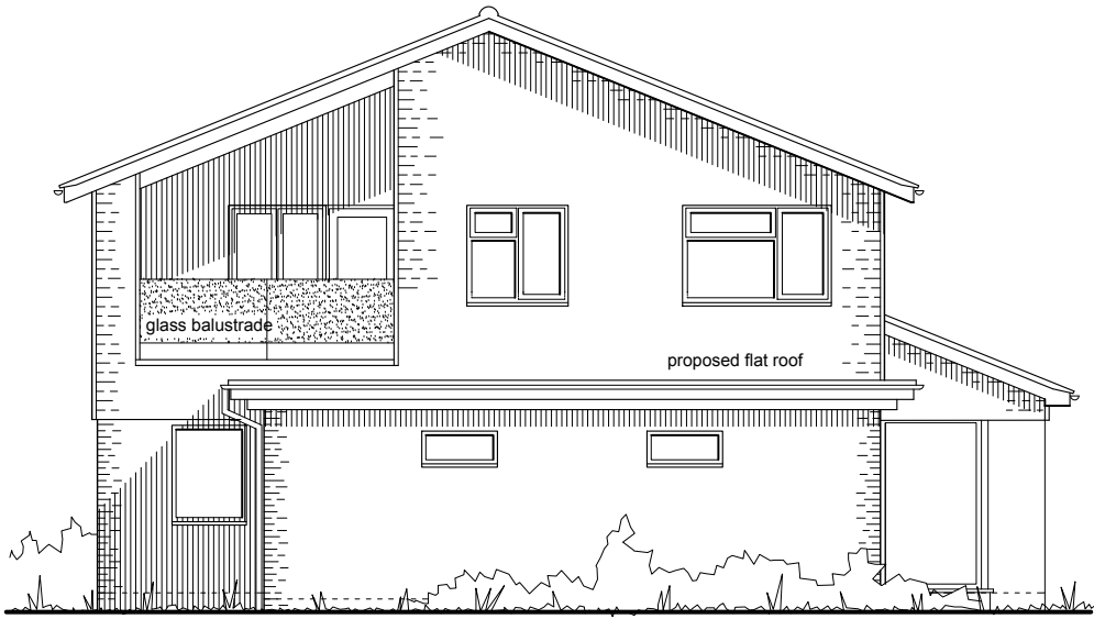
North Elevation
