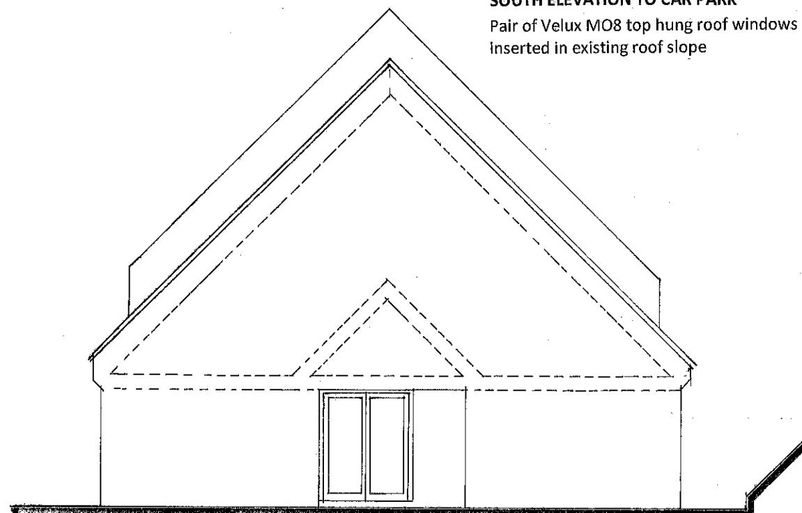
EAST ELEVATION
