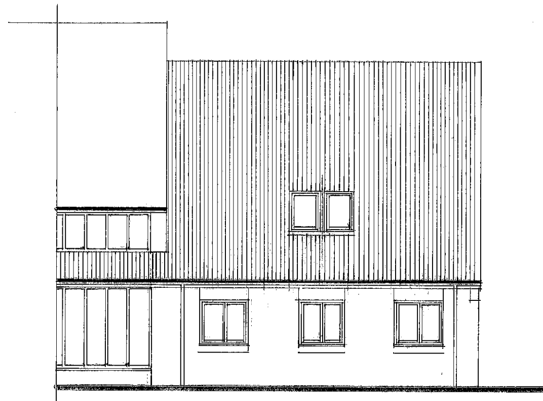
SOUTH ELEVATION TO CAR PARK Pair of Velux MO8 top hung roof windows Inserted in existing roof slope
