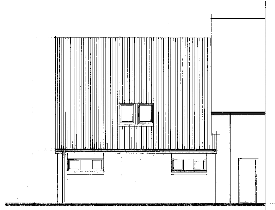
NORTH ELEVATION TO CHURCHYARD Pair of Velux MO8 top hung roof windows Inserted in existing roof slope
