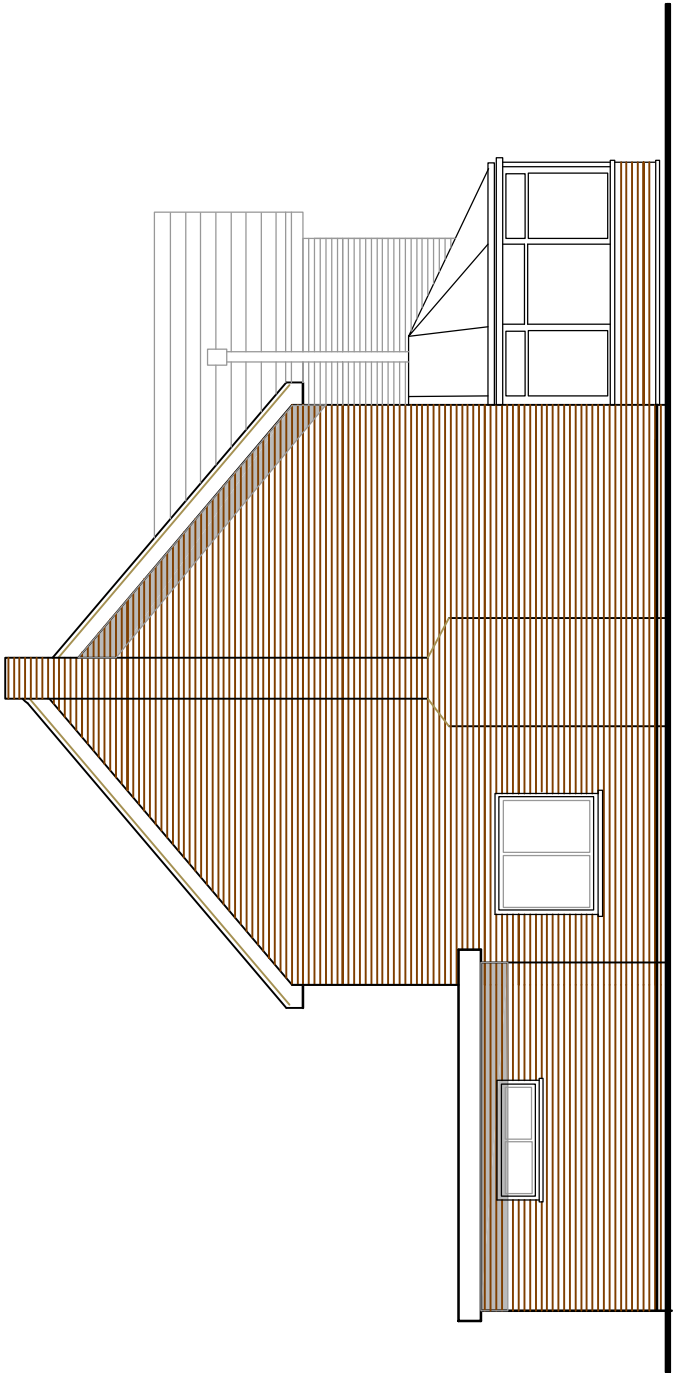
PROPOSED WEST ELEVATION 1:100
