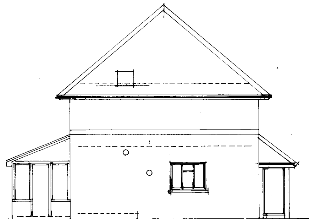
NORTH ELEVATION TO 10 WANSFORD WAY
