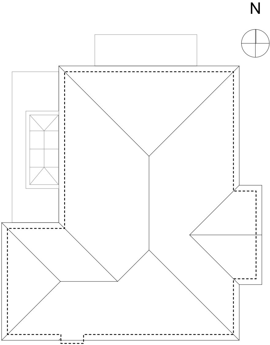
PROPOSED ROOF PLAN | 1:100@A3
