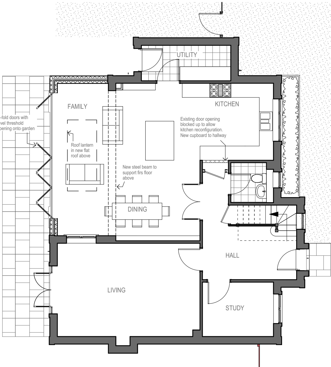
PROPOSED GROUND FLOOR | 1:100@A3
