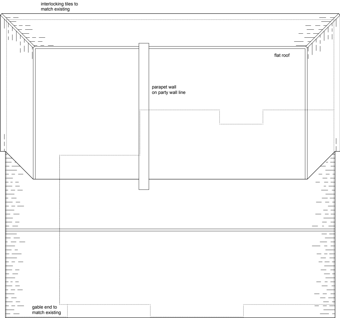
Roof Plan
