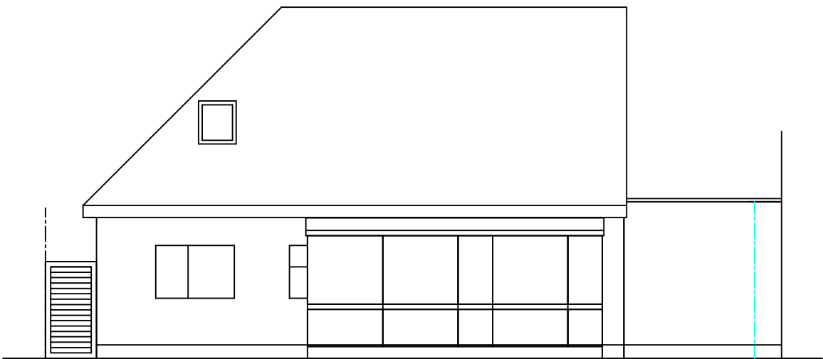
Existing Rear Elevation (West)
