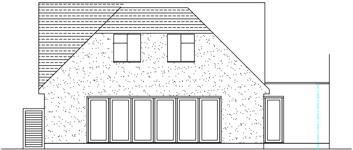
Proposed Rear Elevation (West)
