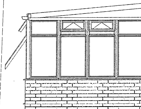
WEST ELEVATION
