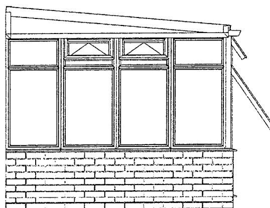
EAST ELEVATION
