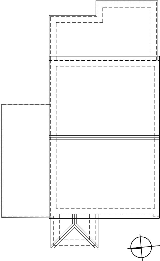
Roof Plan
