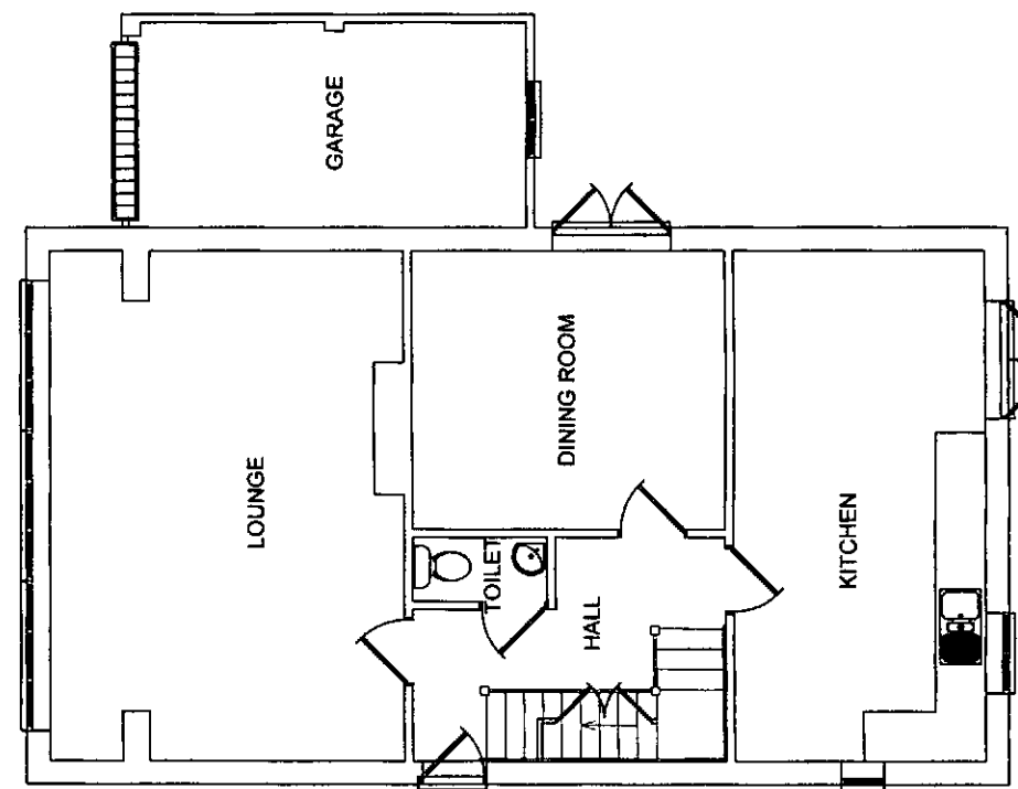
NEW GROUND FLOOR PLAN
