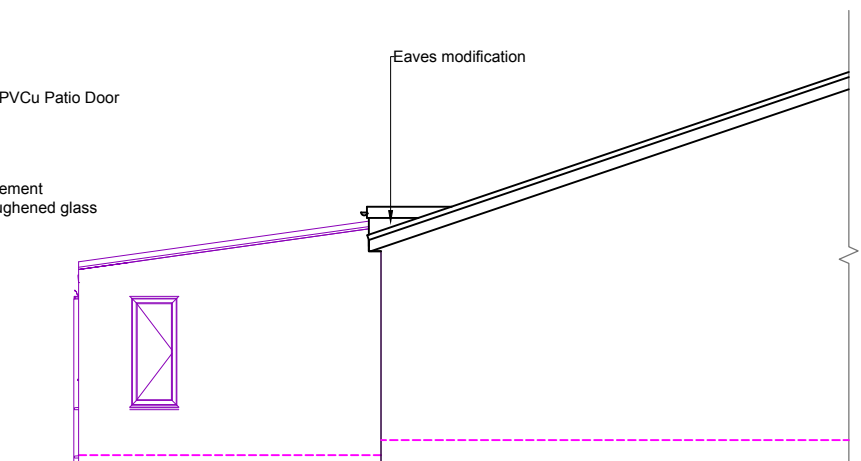
Proposed left elevation
