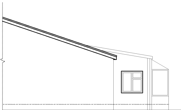
Existing right elevation
