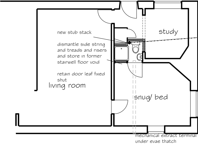
Part Ground Floor Plan Proposed
