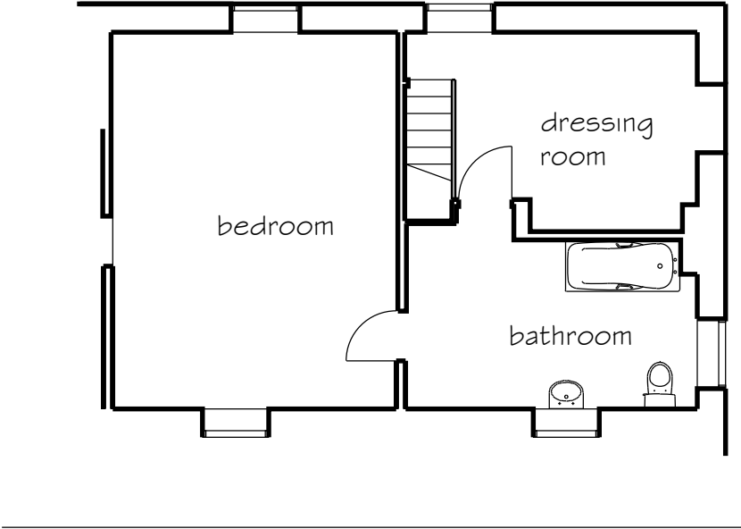
Part First Floor Plan Existing
