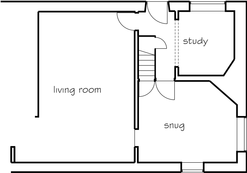
Part Ground Floor Plan Existing
