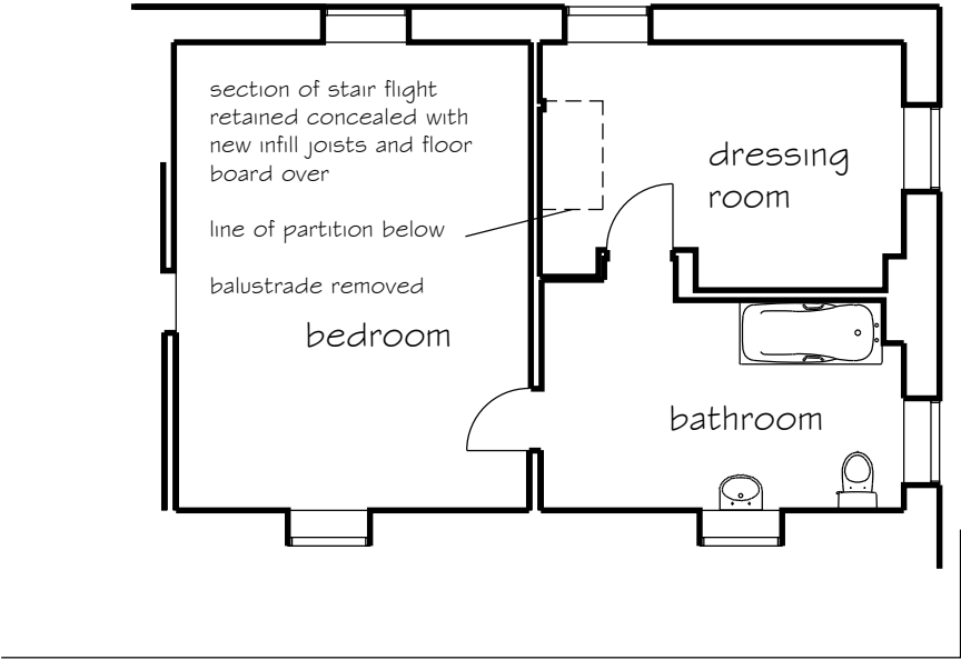
Part First Floor Plan Proposed
