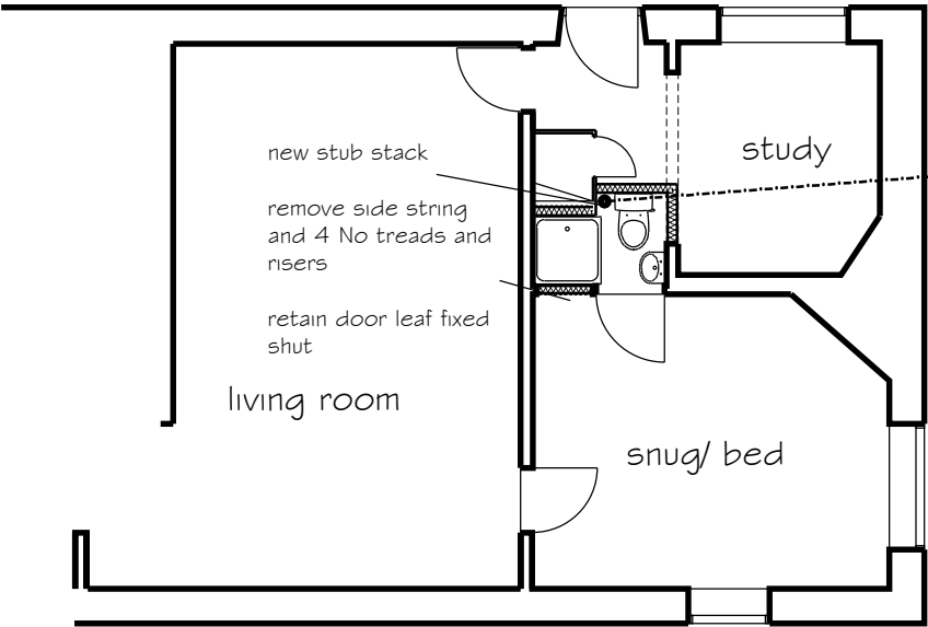
Part Ground Floor Plan Proposed
