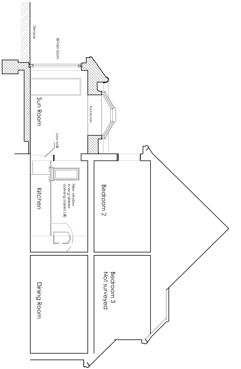
Cross-Section AA
