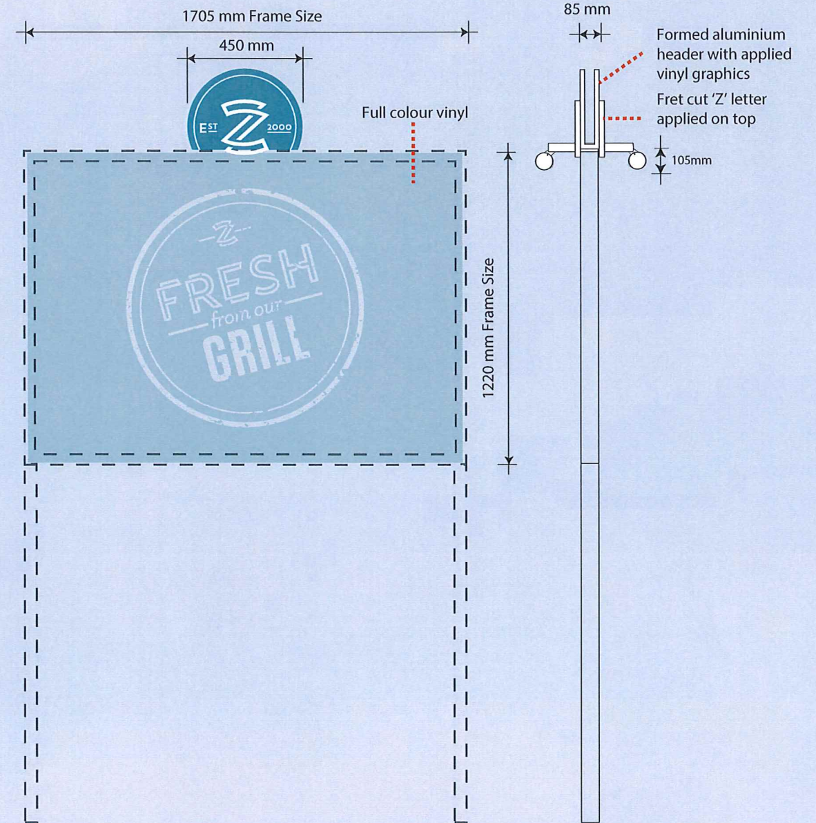
ITEM 10 Existing sign and post to be repainted with the addition of a New sizzle icon applied to top of the existing landscape sign. Existing trough light illumination to be retained. AGL: 1380mm Scale 1:20
