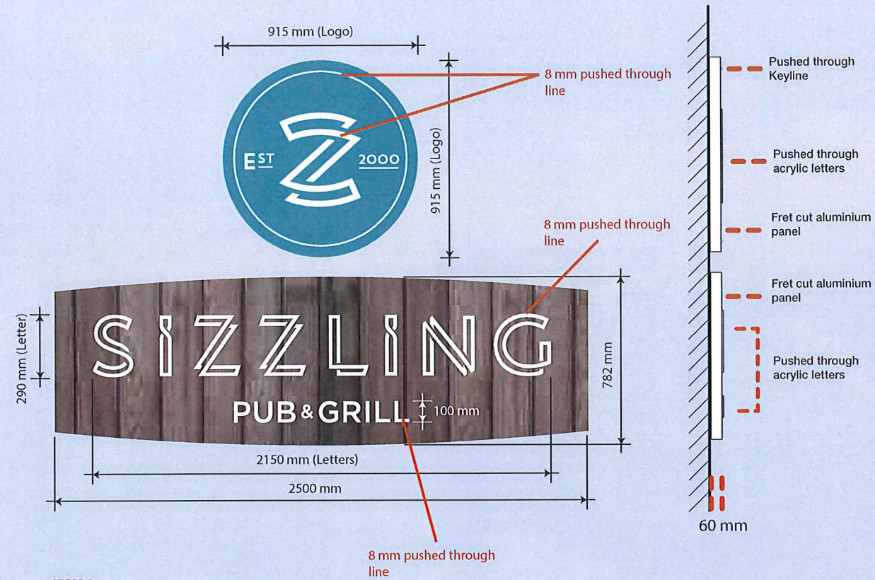
ITEM 6 An internally illuminated logo, with push through letters. With a set of individual, internally illuminated, pushed through letters. All mounted to a backboard, with timber cladding effect vinyl. AGL: 3200mm Scale 1:25 @ A3
