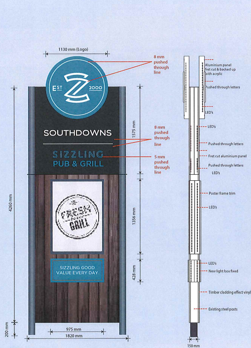
ITEM 4 ( 1 off) REFURBISHMENT OF EXISTING TOTEM SIGN Double sided totem sign. Logo - An internally illuminated logo, with a pushed through 'Z' letter & outer circle. The smaller letters to be fret cut & backed up in acrylic. Main panel - An internally illuminated fret cut panel. And a set of individual pushed through letters. Light box panel - An internally illuminated image panel. Steel posts. With timber cladding effect vinyl. Scale 1:40 AGL:0
