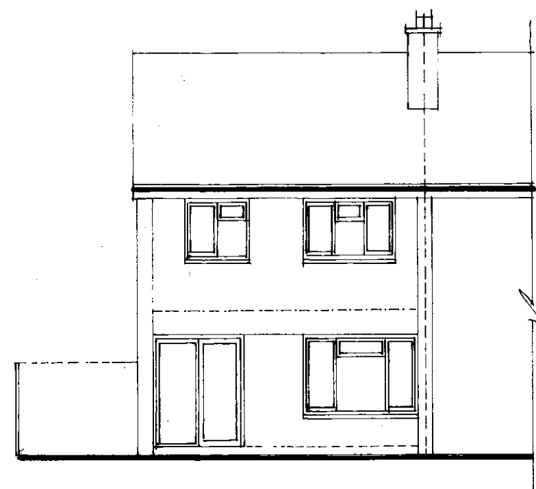
SOUTH ELEVATION TO BALA CRESCENT
