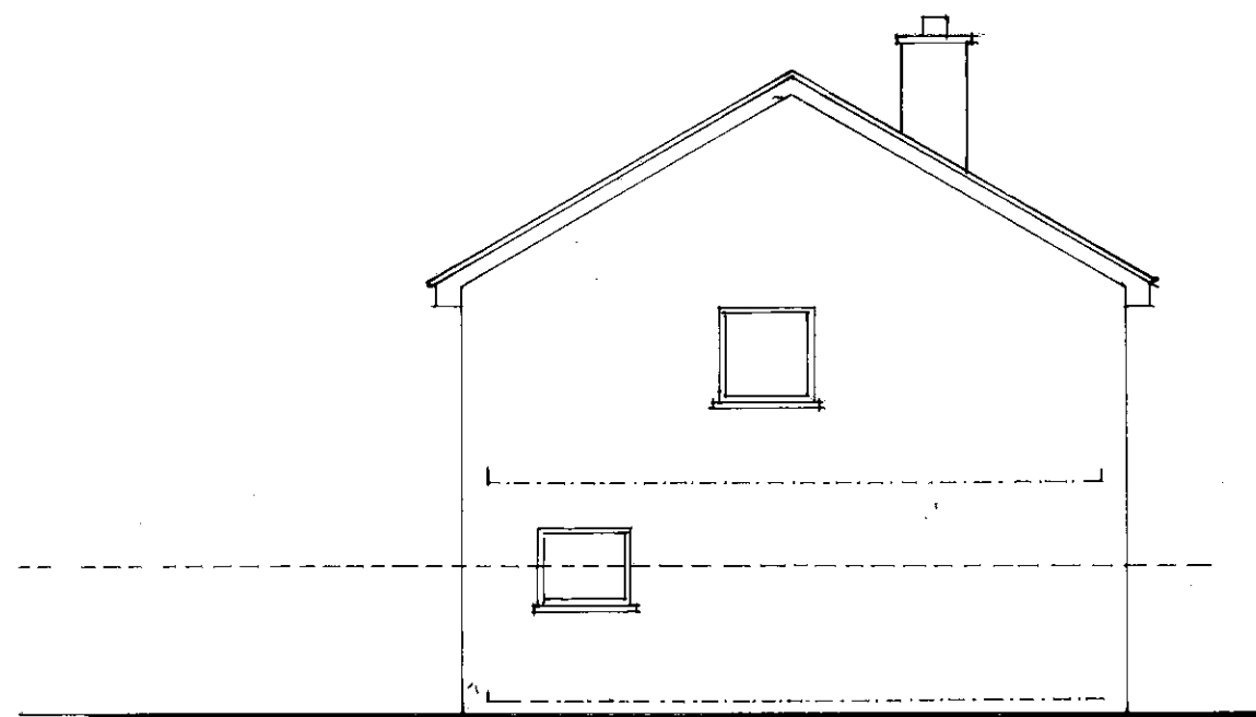
WEST ELEVATION
