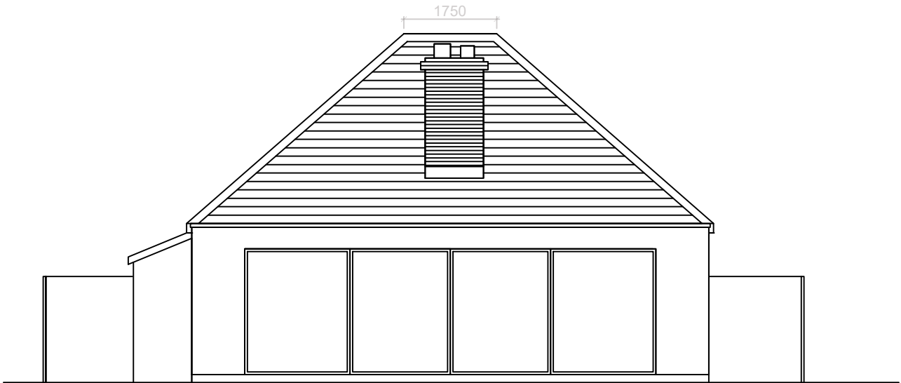
EXISTING REAR (SOUTH) ELEVATION
