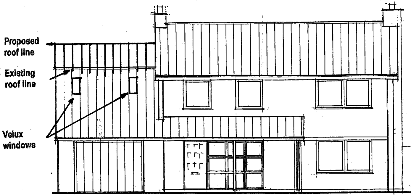
FRONT ELEVATION
