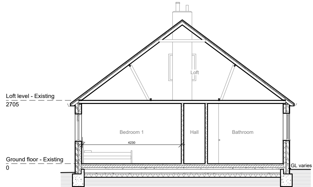
2 Cross section - Existing 1:100
