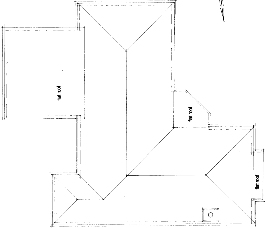
ROOF PLAN PLAN 1:100
