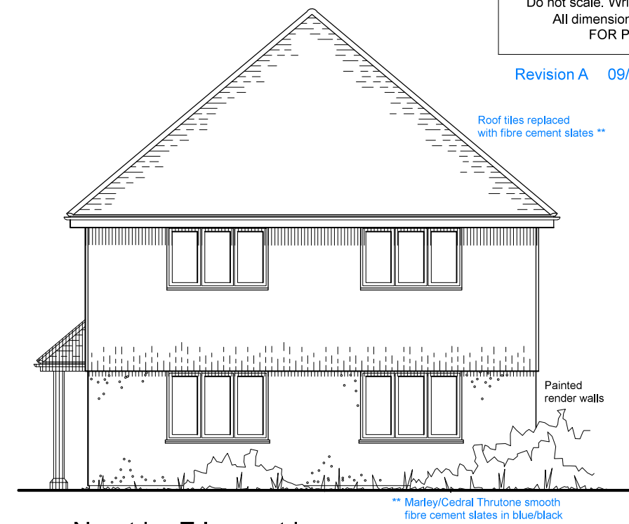
North Elevation
