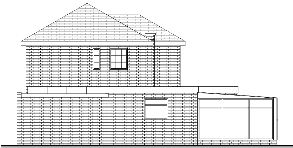
Existing North Elevation 1 : 100
