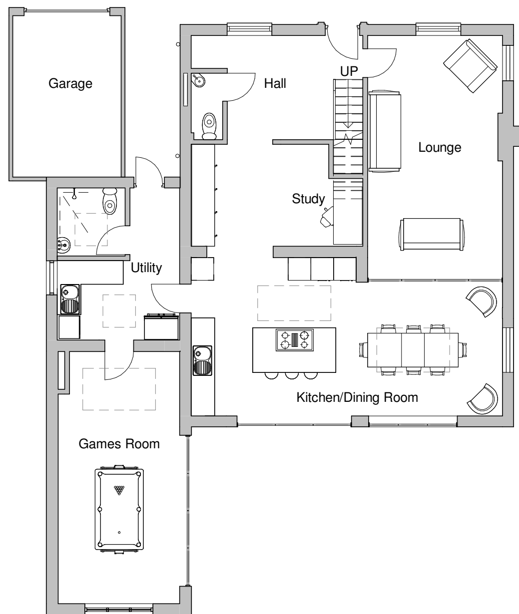
Proposed Ground Floor 1 : 100
