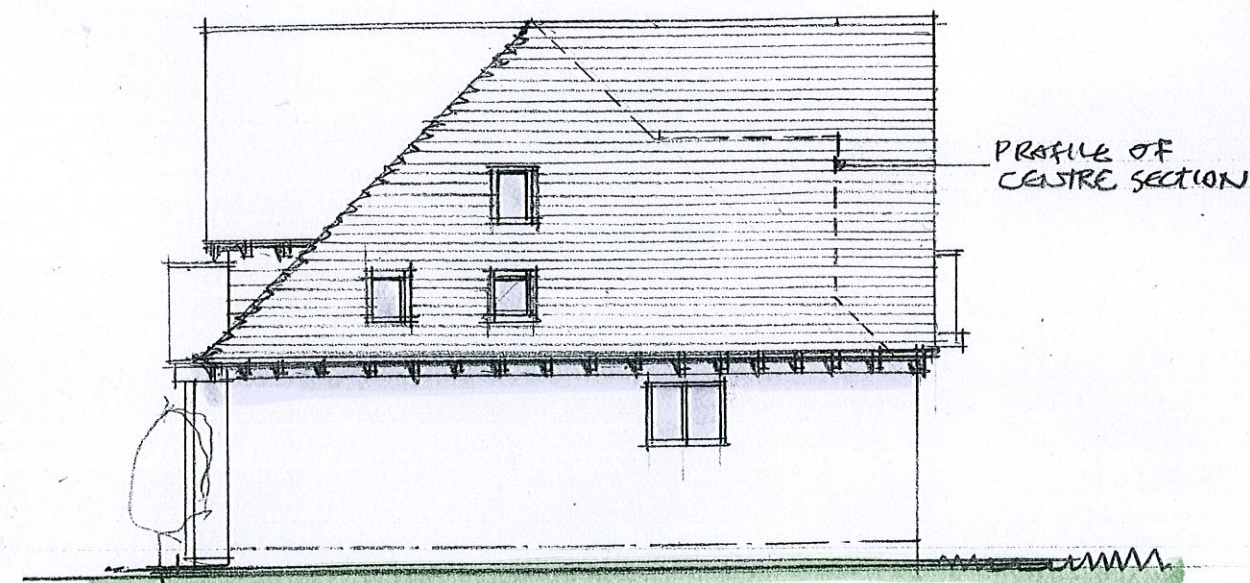
WEST ELEVATION
