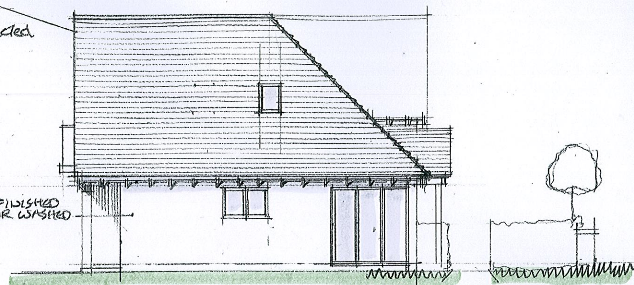
FLANK EAST (TO WEDGWOOD RD, (LB BOUNDARY WALL & PLANTING NOT SHOWN))
