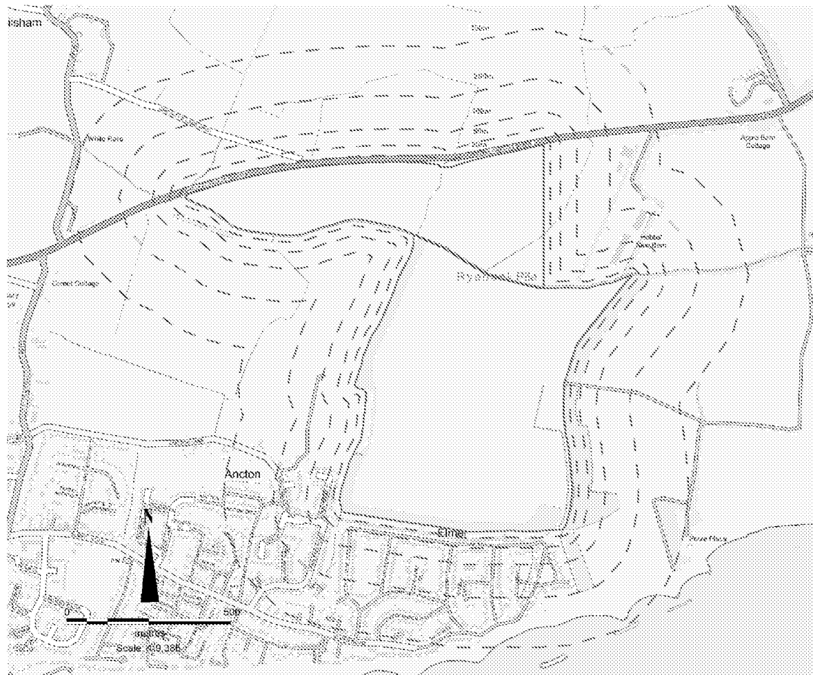
Figure 11.3.1: Site B Construction Buffers
