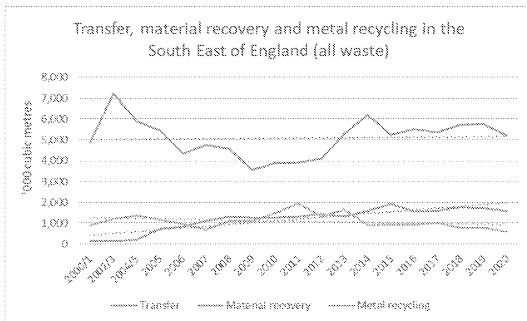
Figure 17-1 Transfer, materials recovery and recycling in the South East of England region (2000/1 – 2020)
