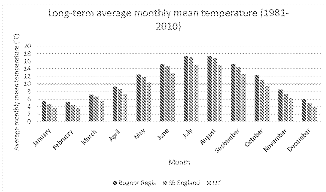
Figure 16-2 Long-term average mean monthly temperature for SE England region and Bognor Regis weather station, by comparison with the UK. Source: Bognor Regis (West Sussex) UK climate averages - Met Office
