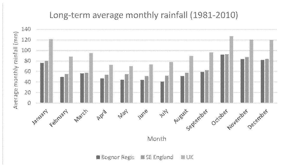
Figure 16-1 Long-term average monthly rainfall in areas of Bognor Regis, SE England and the UK within the period of 1981-2010)
