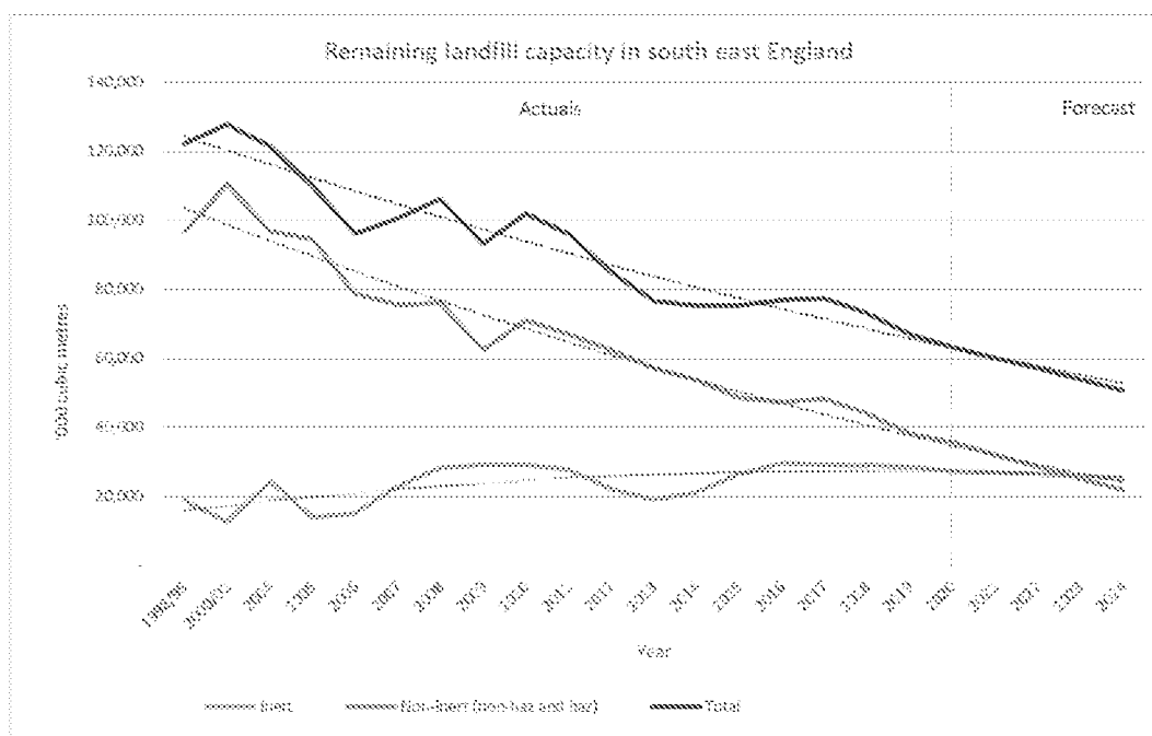
Figure 17-3 Remaining landfill capacity in South East of England
