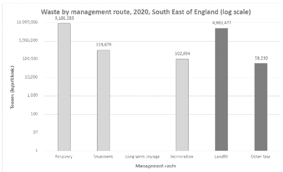
Figure 17-2 Construction and demolition waste management by route for the region
