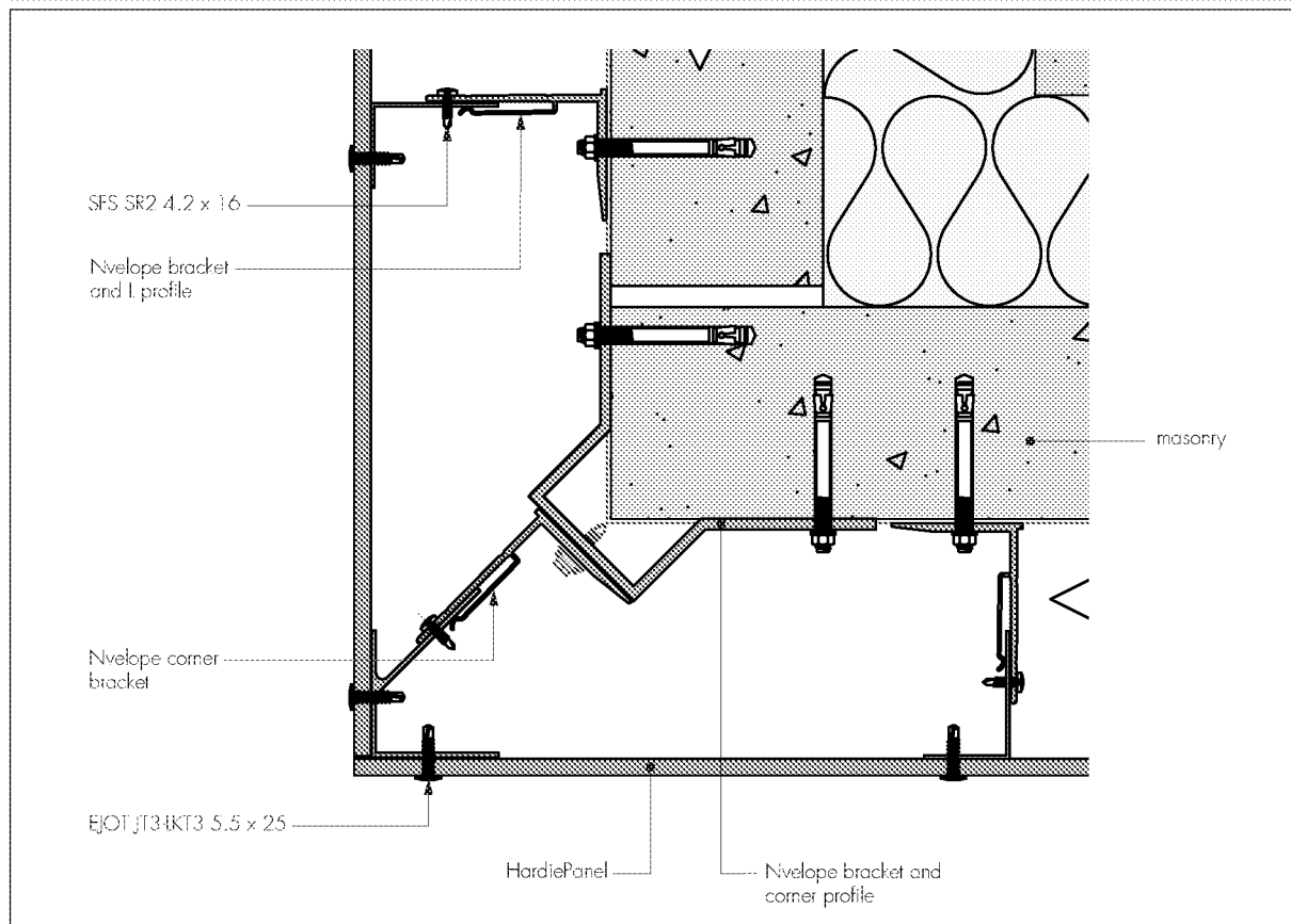
Figure 10 Concealed corner detail on metal framing
