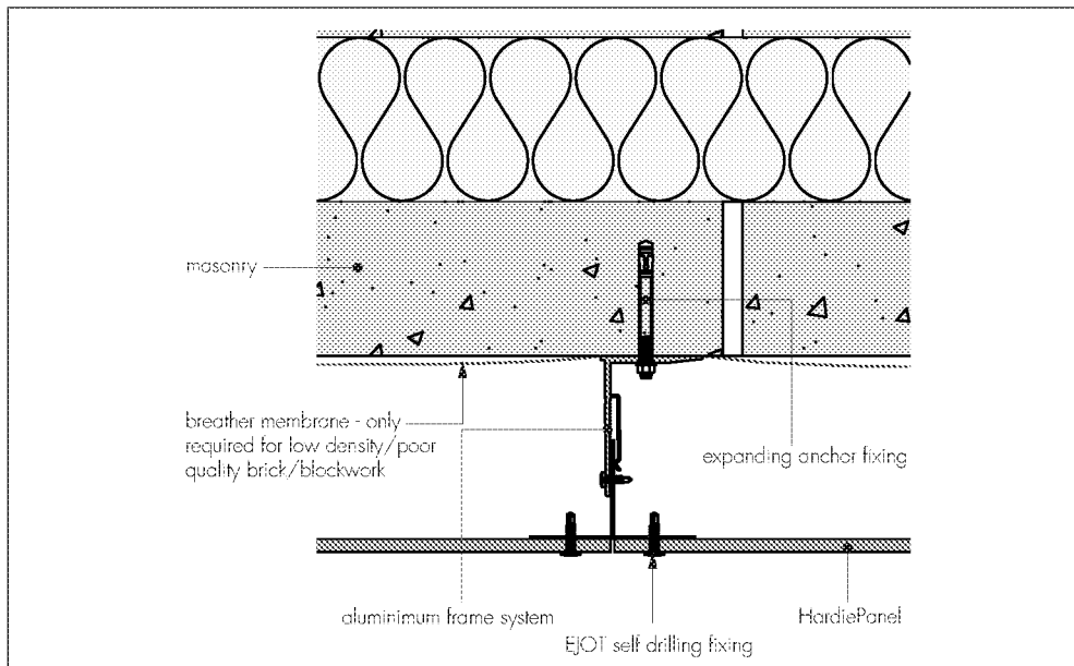
Figure 8 Vertical joint on masonry — metal frame
