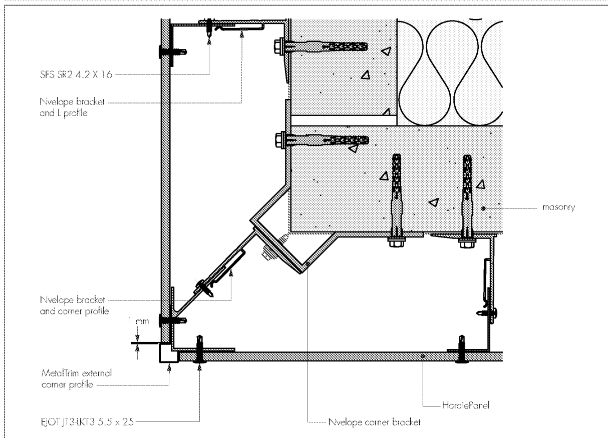
Figure 9 Corner detail on metal framing using MetalTrim external corner
