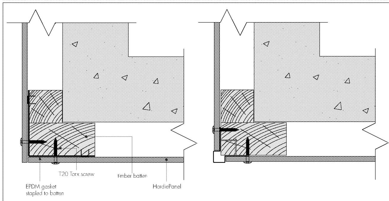
Figure 6 Corner detail on timber frame
