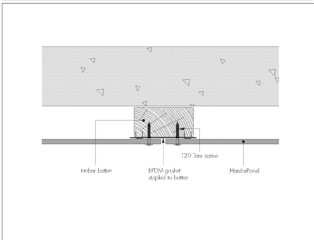
Figure 5 Vertical jointing on masonry wall — timber frame
