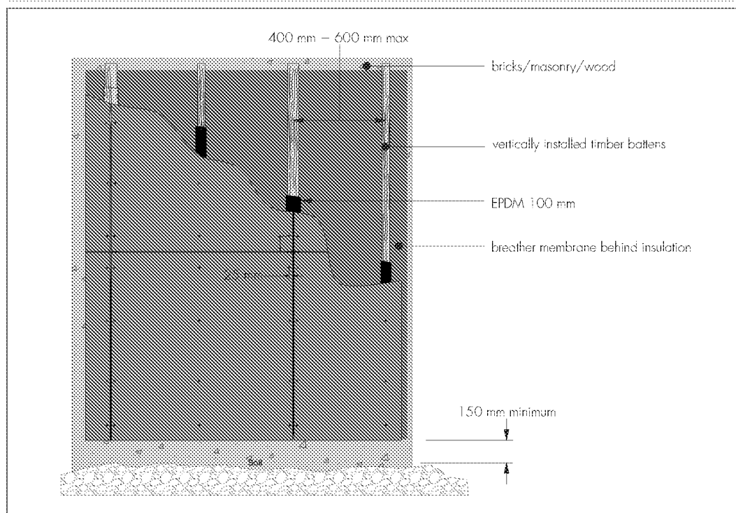
Figure 3 Fixing detail on timber frame
