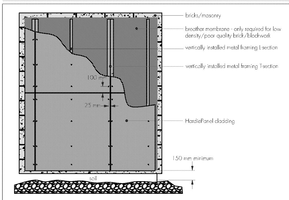
Figure 7 Fixing detail on metal frame
