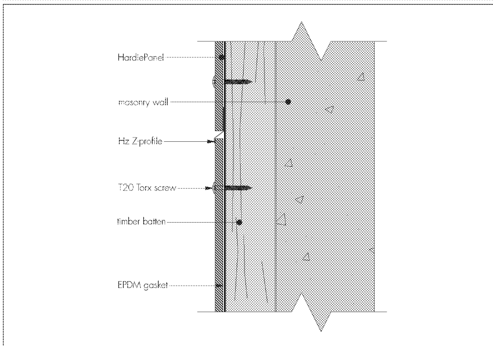
Figure 4 Horizontal jointing detail — timber batten
