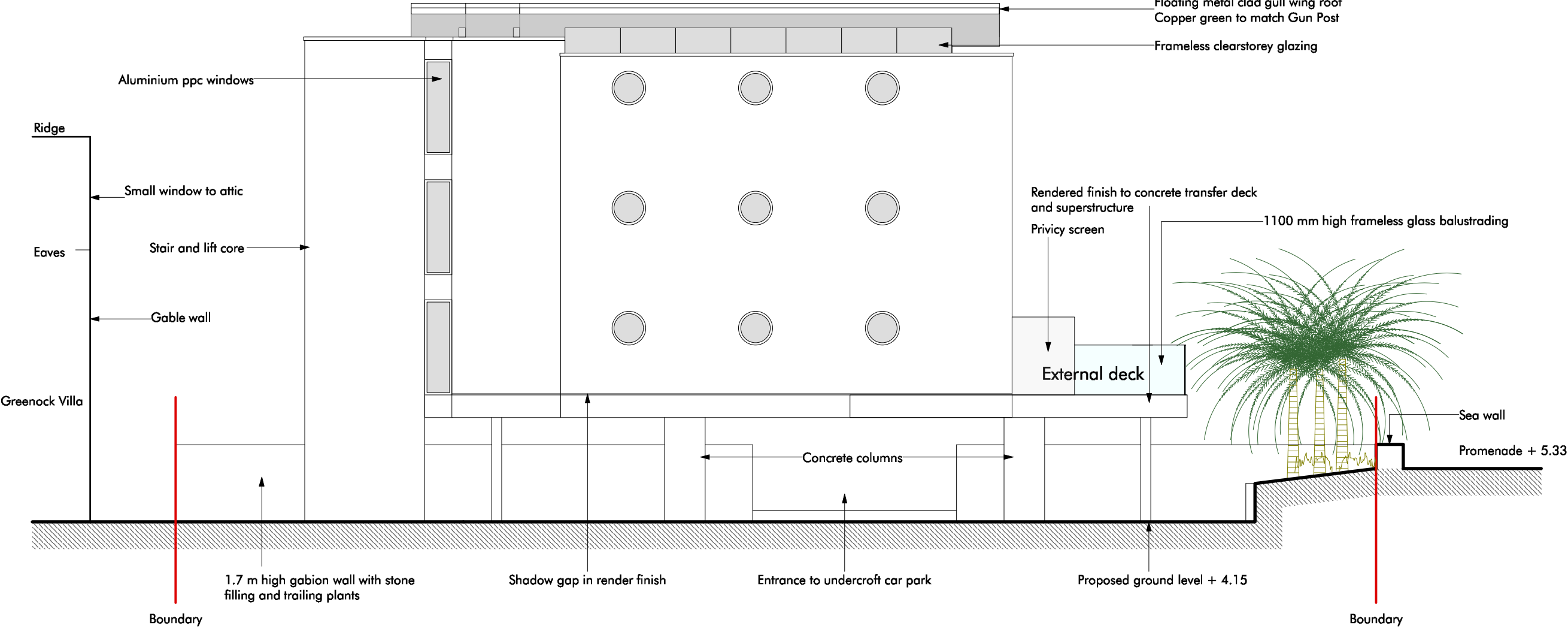
Side Elevation (South)
