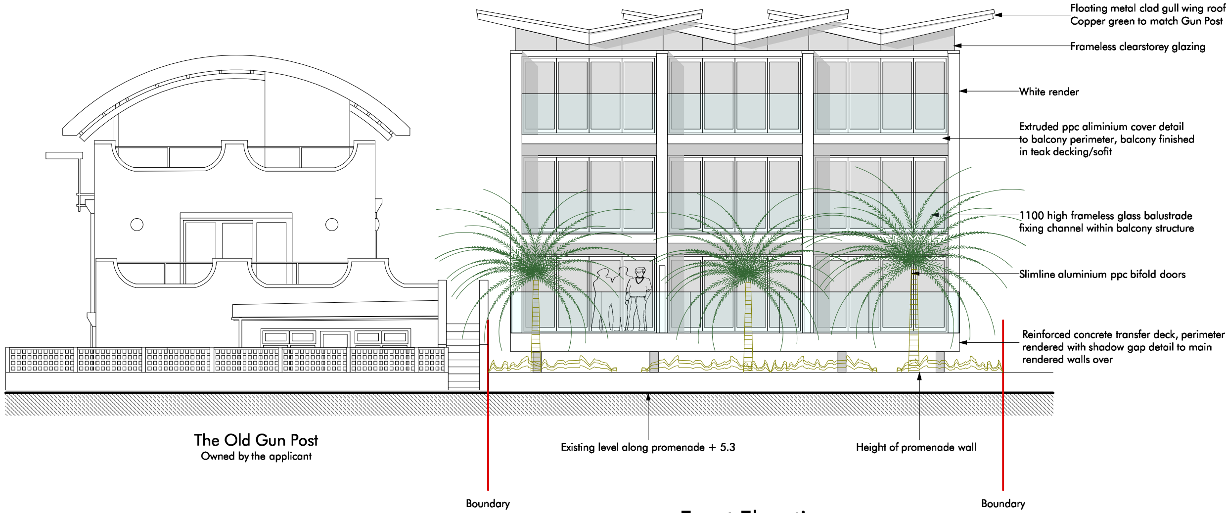
Front Elevation From Promenade (East)
