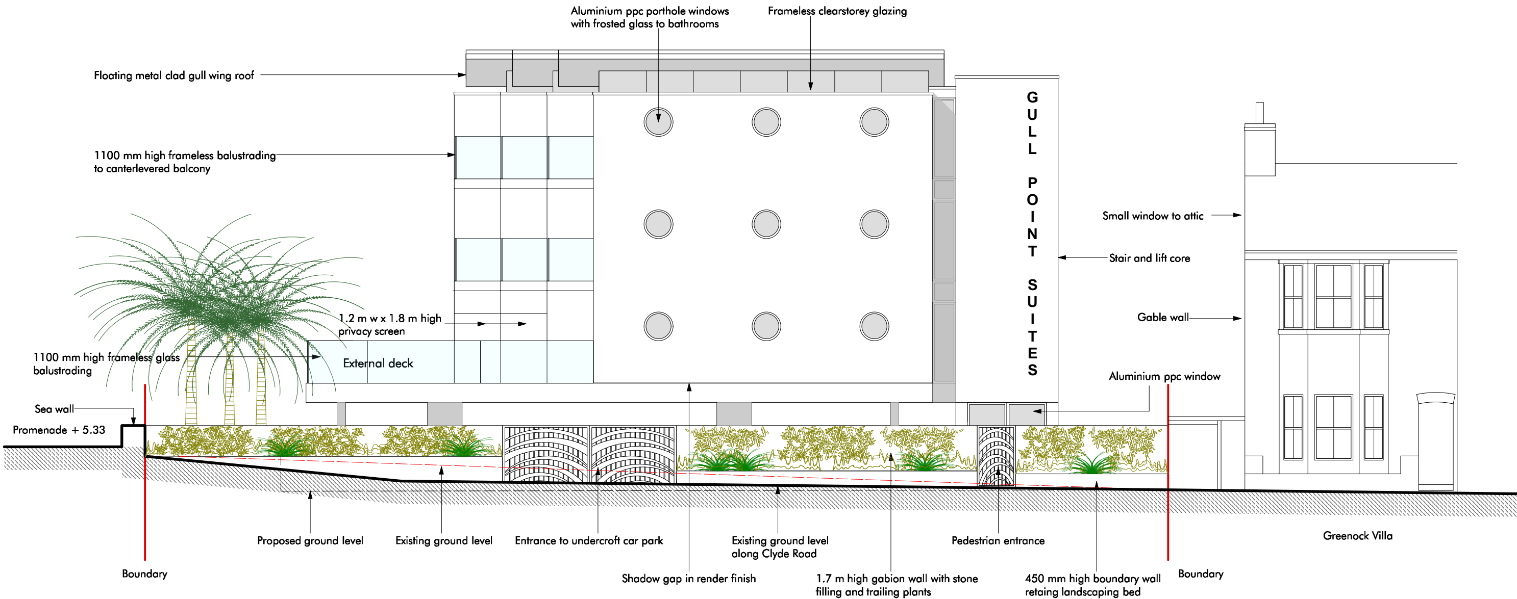
Elevation to Clyde Road (North)
