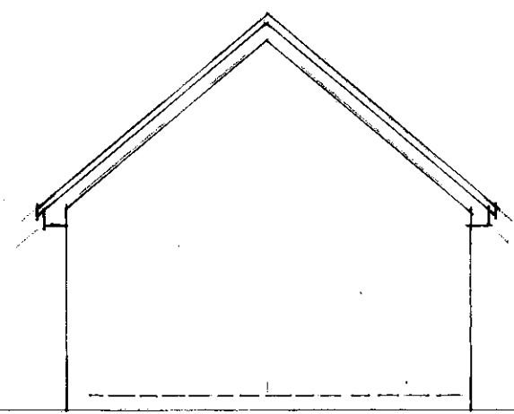
WEST ELEVATION
