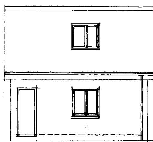
SOUTH ELEVATION
