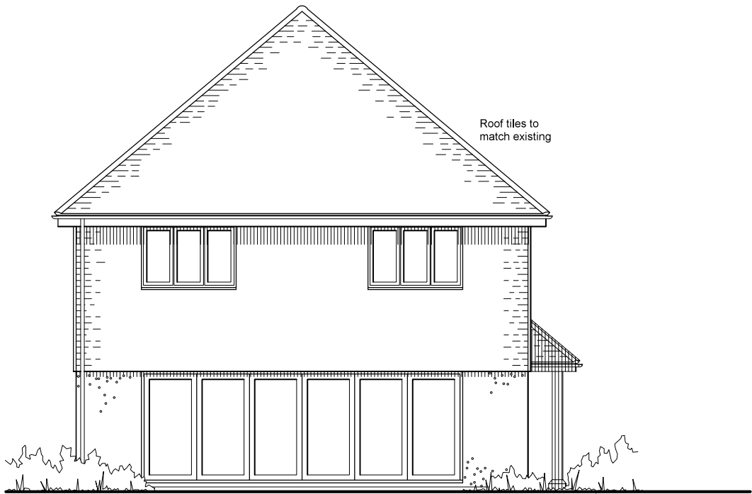
South Elevation
