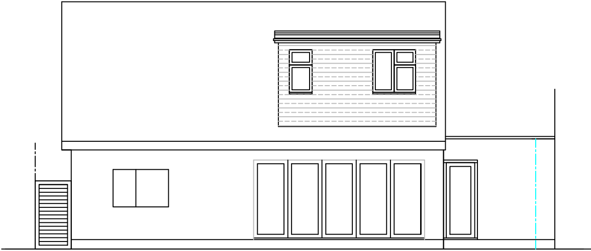
Proposed Rear Elevation (West)
