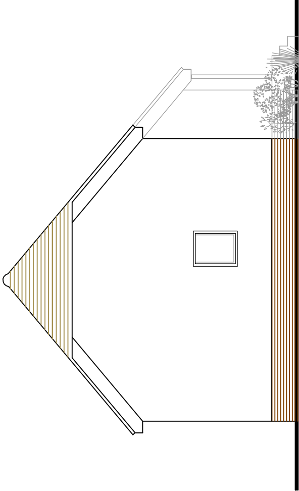
PROPOSED WEST ELEVATION 1:100
