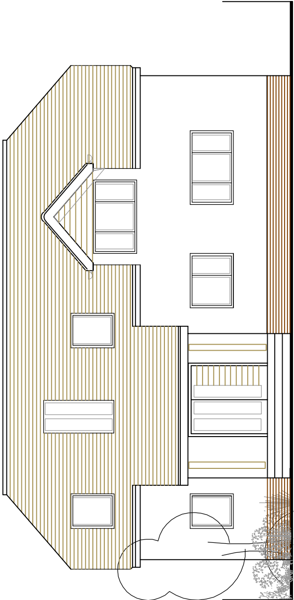
PROPOSED SOUTH ELEVATION 1:100
