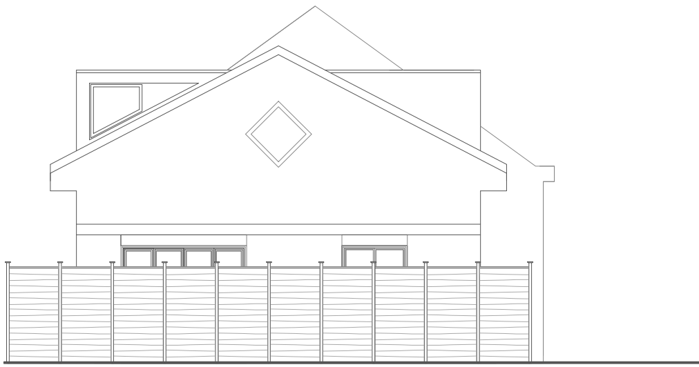
North Elevation Block A - Proposed 1:100
