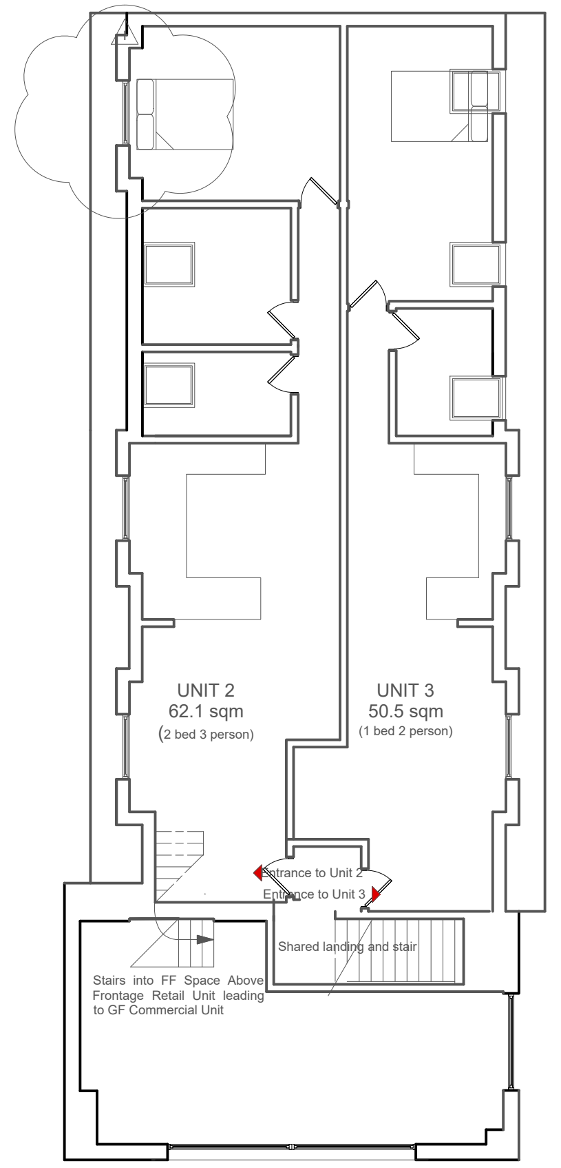
First Floor Plan - Proposed 1:100
