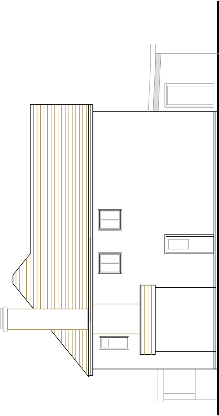
PROPOSED EAST ELEVATION 1:100
