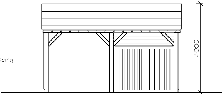
South Elevation
