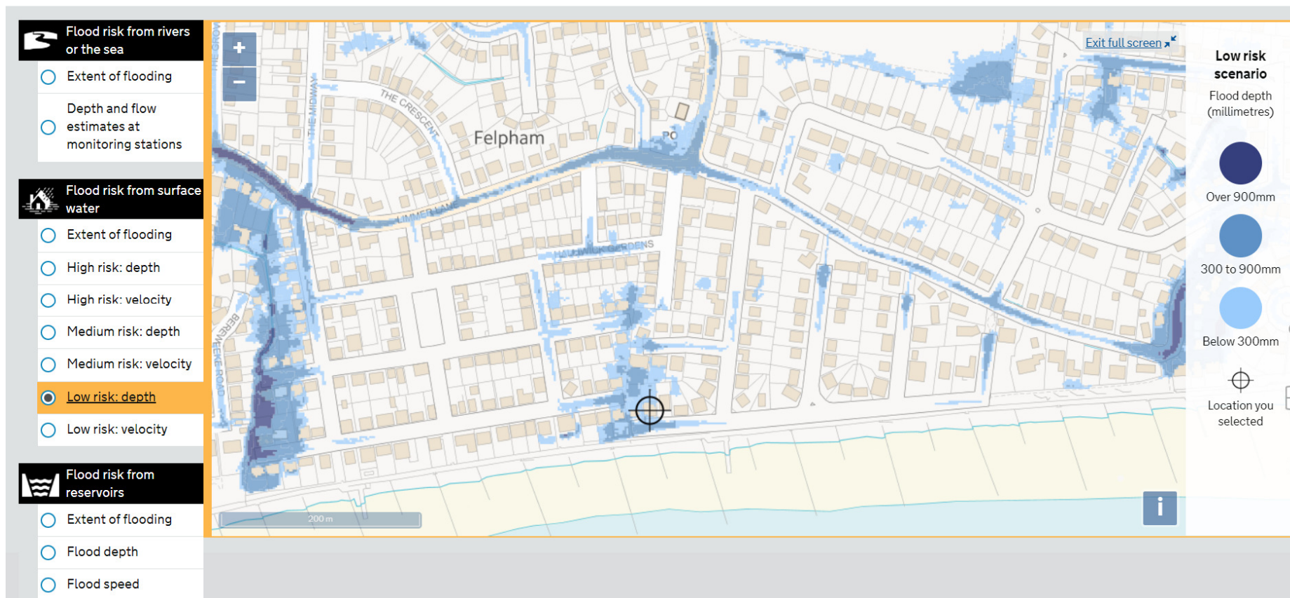
PO22 7LH – Flood Risk from Surface Water - Depth
