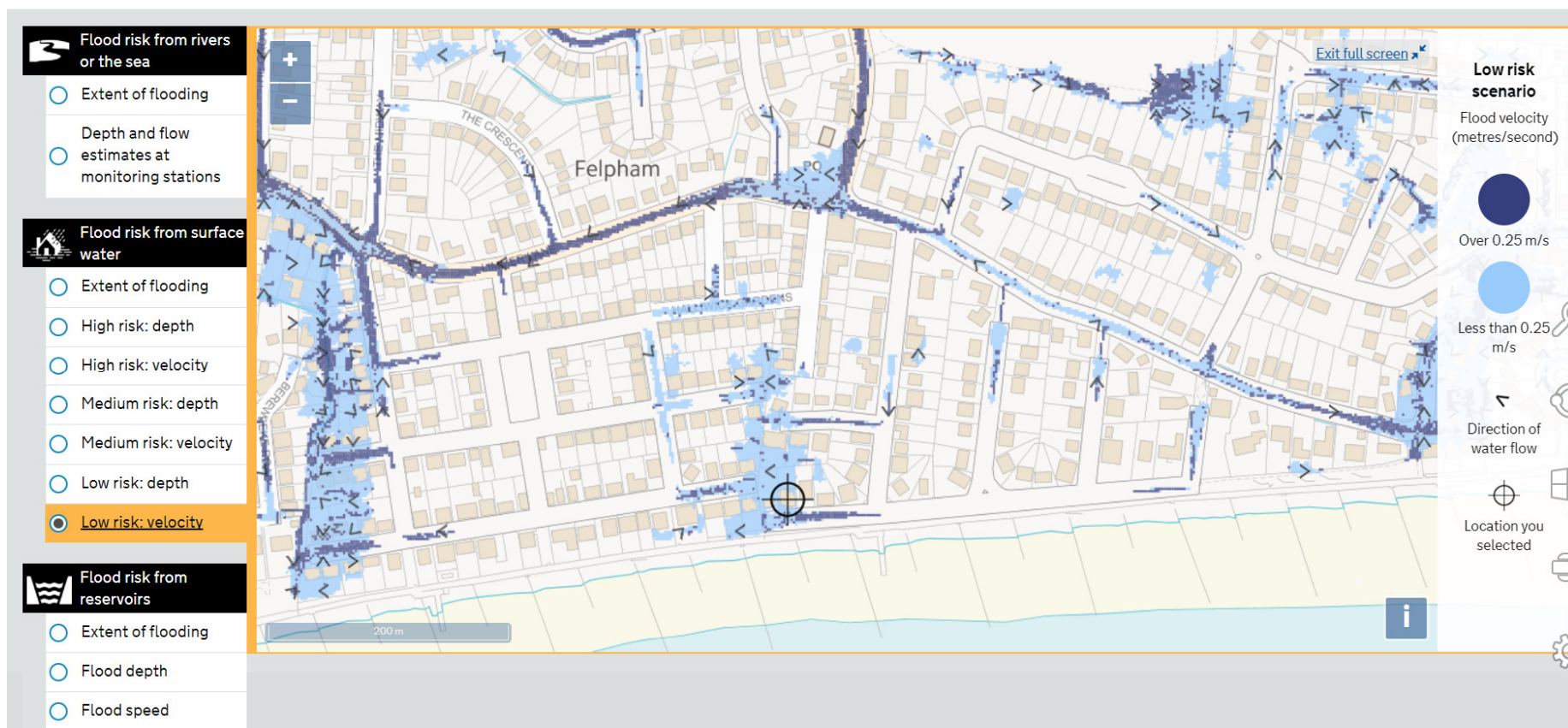
PO22 7LH – Flood Risk from Surface Water - Velocity
