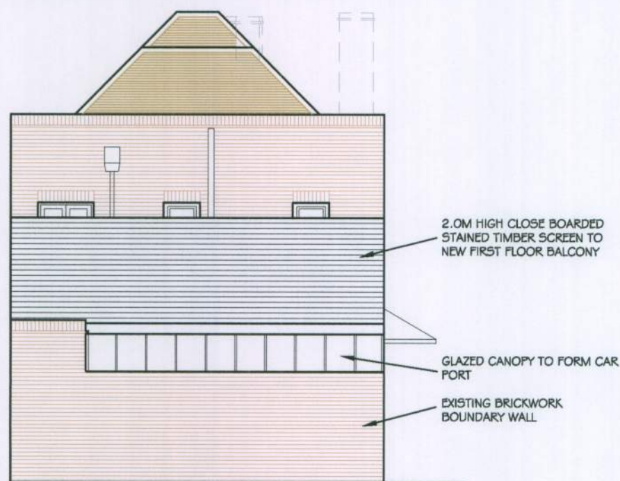
PROPOSED EAST ELEVATION (SHOWING BALCONY AND CAR PORT)
