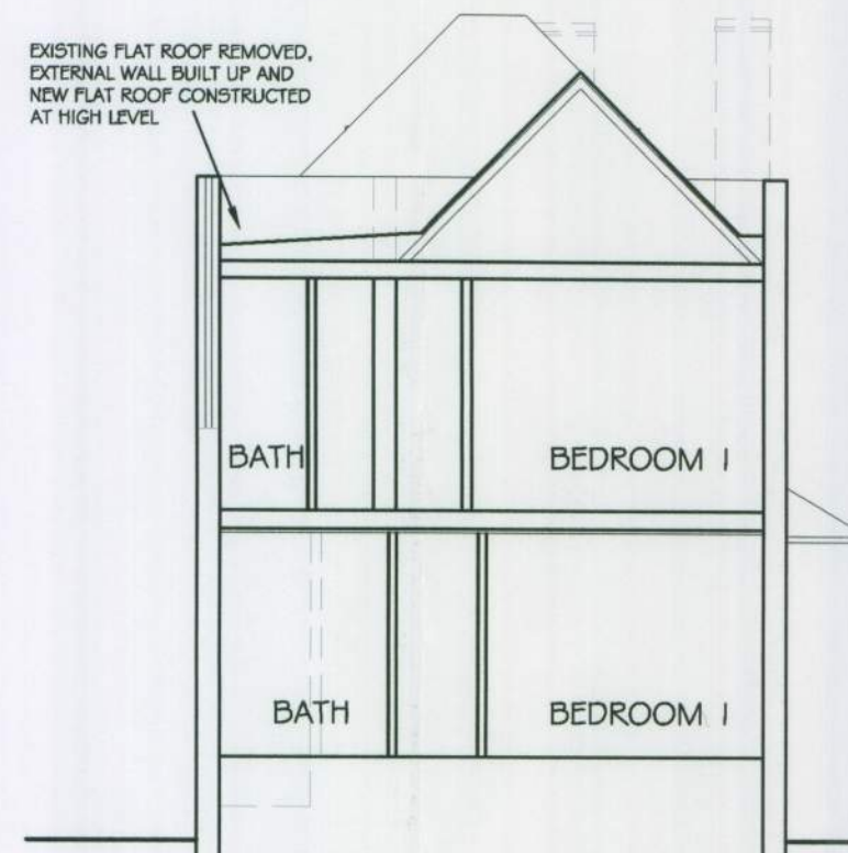
PROPOSED SECTION A-A
