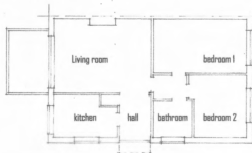
EXISTING FLOOR PLAN 1:100
