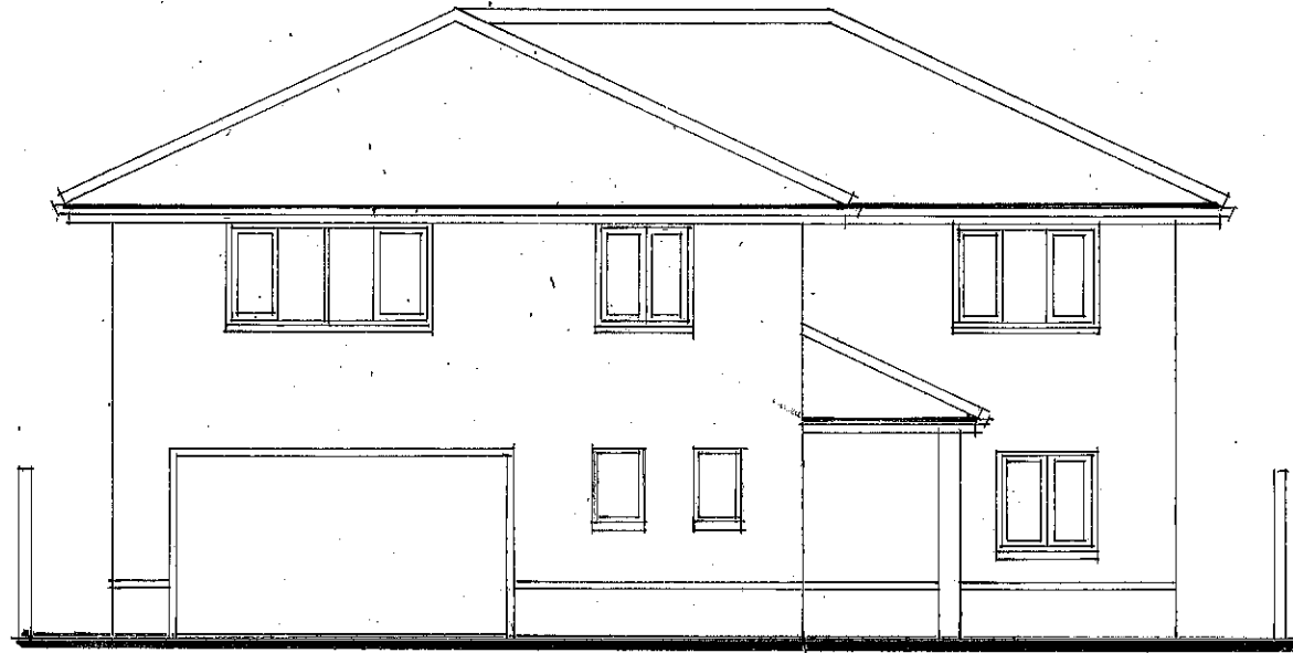
WEST ELEVATION TO LIMMARD WAY
