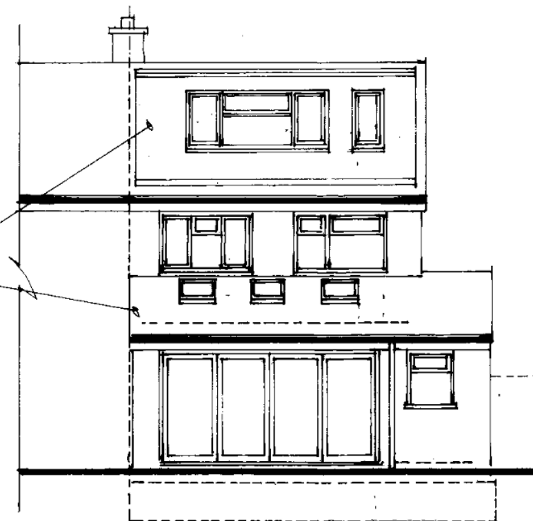
NORTH ELEVATION TO REAR GARDEN
