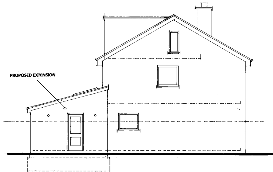
WEST ELEVATION TO 16 BALA CRESCENT
