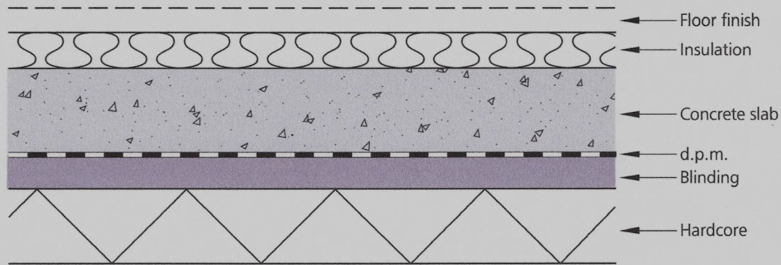
Figure 6.4 Ground-supported floor – Preferred option
